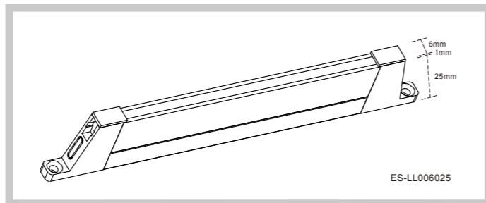
Aluminum Profile For LED Side View LED Strip
