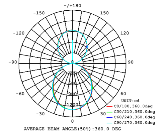
Illumination Curve and Luminous Intensity Distribution Diagram 4000K(4 Feet)
