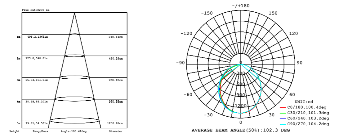
ILLUMINATION CURVE AND LUMINOUS INTENSITY DISTRIBUTION DIAGRAM 4000K(4 FEET)
