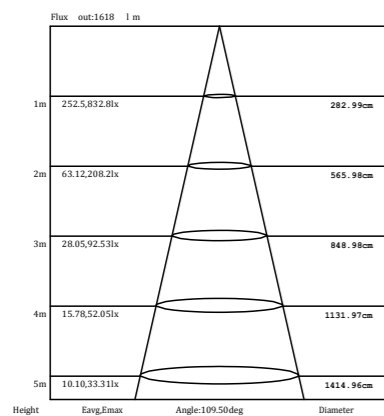
Illumination Curve and Luminous Intensity Distribution Diagram 4000K(4 Feet)
